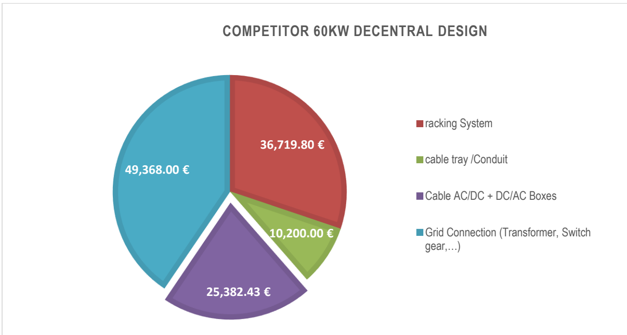
Figure 7: BOS costs for the 60-kW competitor inverter installation
